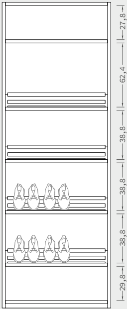
1 ripiano 4 ripiani inclinati porta scarpe 1 shelf 4 inclined shoes rack shelves
