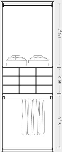
2 ripiani 1 tubo appendiabiti 1 porta pantaloni estraibile 2 shelves 1 coat-hanger 1 removable trousers rack
