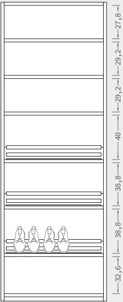
3 ripiani 3 ripiani inclinati porta scarpe 3 shelves 3 inclined shoes rack shelves
