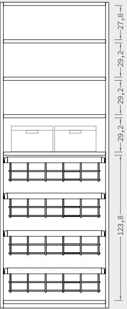
4 ripiani 4 cassetti in filo estraibili 4 shelves 4 removable drawers
